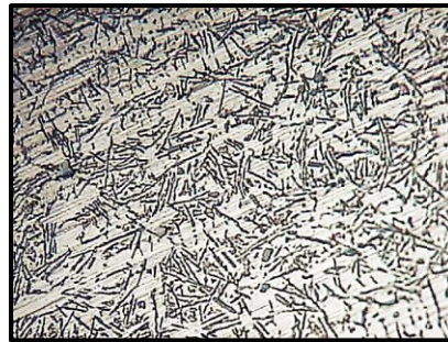
Figure. 2 shows the microscopic images of the unmodified Aluminum-11% Silicon alloys at 0 % Sb and 125 X
