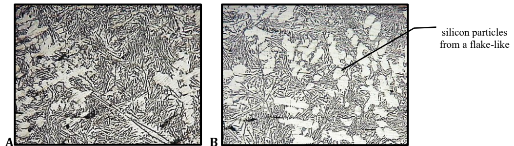
Figure. 3 shows the microscopic images of the amended Aluminum-11% Silicon Alloys, A: 0.05 % Sb at 125 X and B: 0.1 % Sb at 125 X
