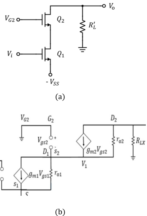
Figure 5. Cascode PA configuration (a) schematic diagram and (b) small signal equivalent circuit[54].
