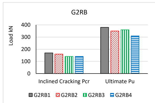
Figure 11: Ultimate and Cracking Load for First Group
