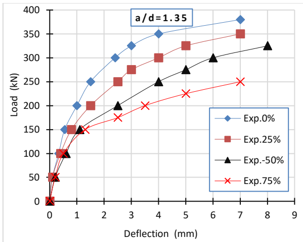
Figure 15: Load versus mid-span deflection curve for G2RB
