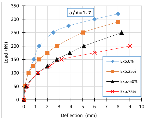
Figure 16: Load versus mid-span deflection curve for G3RB
