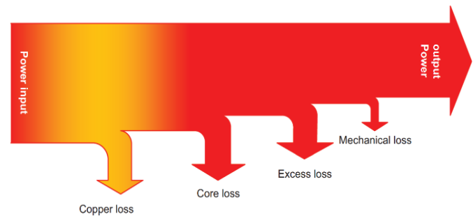
Figure1. Distribution losses in SRM.
