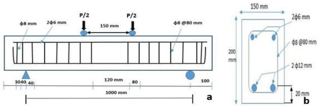
Reinforcement Details (a) Longitudinal View (b) Cross Section
