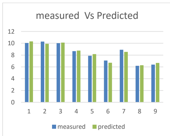
Figure 5. This compares the measured values of the material removal rate with the expected values.
