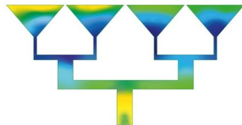
Figure 9. Electric field distribution at 38.6 GHz
