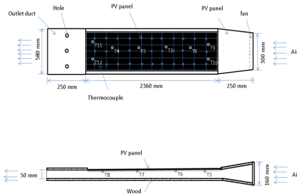
Figure 2. PV/T collector (a) top view, (b) cross-section
