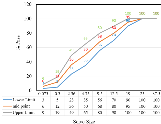
Figure 2: Gradation of aggregate for binder course mixture
