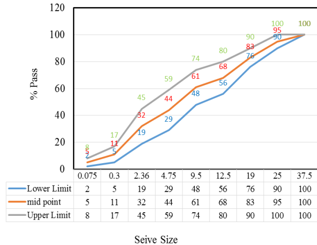
Figure 1: Gradation of aggregate for Base coarse mixture
