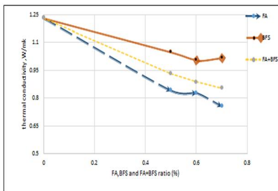
Figure 2. Relationship between mineral admixture and thermal conductivity (Demirboğa et al., 2007).
