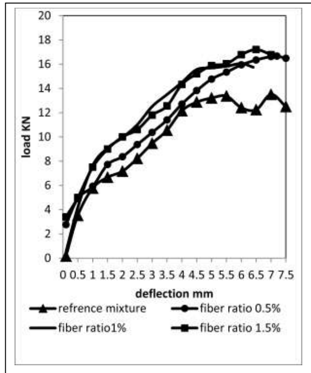
Fig. 9. Load - Deflection curves
