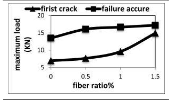
Fig. 8. relationship between fibre ratio and max. load
