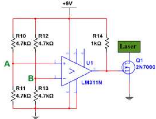
Figure 5. Comparator circuit
