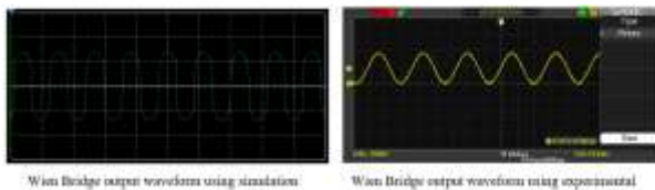
Figure (8). output waveform of simulation and experimental test for Wien Bridge Oscillator.
