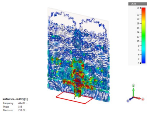
(b) State-2 at 44.4 GHz.
