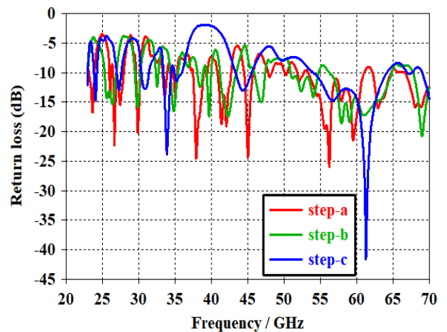
Figure 3: Return loss performances for mm-wave band.
