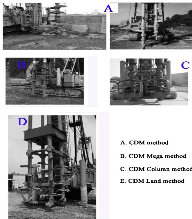
Figure 6. Several kinds of CDM include mixing shafts and blades (Photo is a courtesy of the Cement DMM Association)[6]
